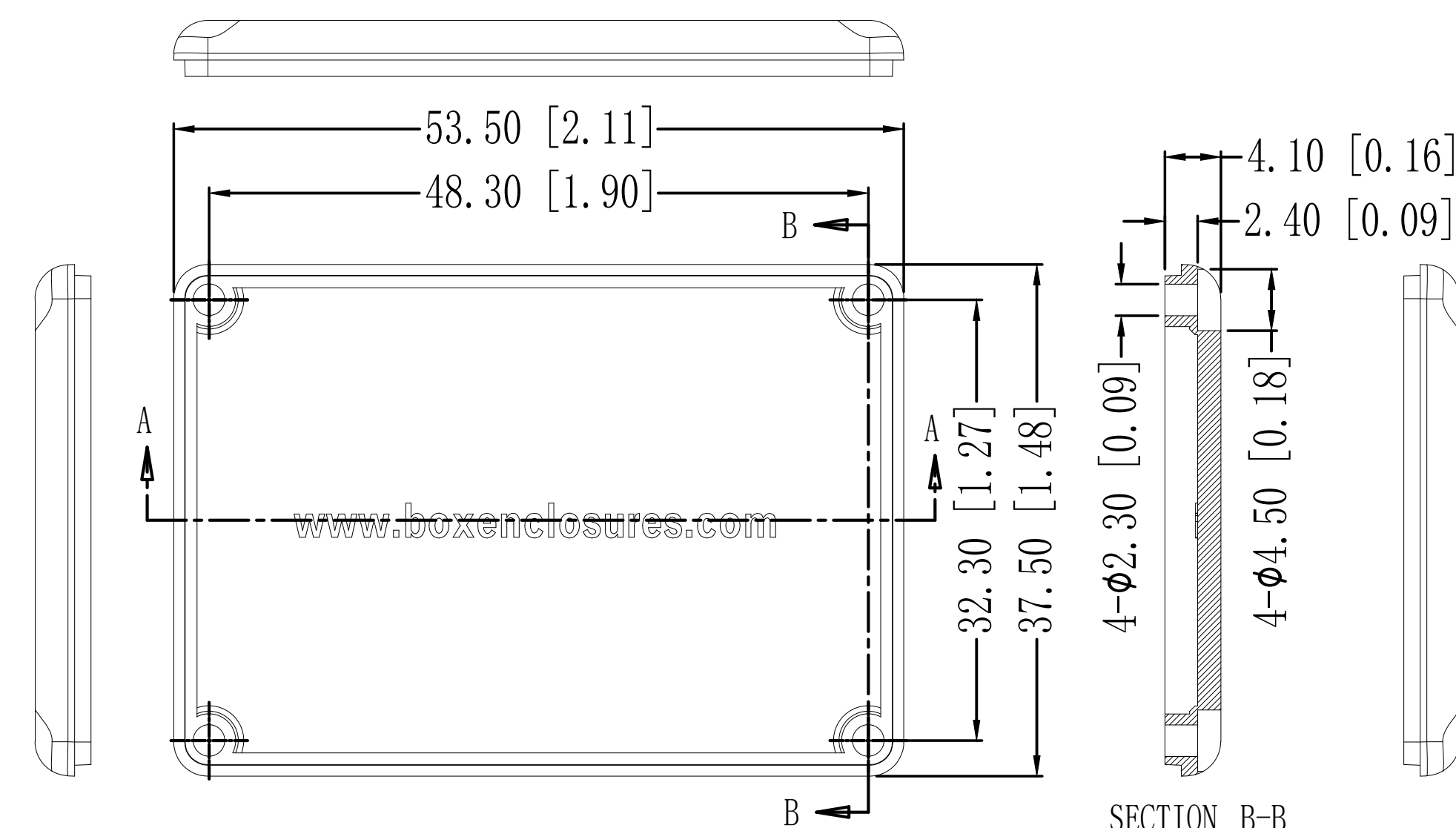
SECTION B-B
