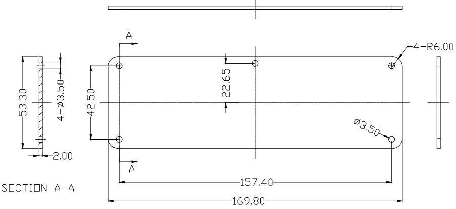
END PLATE
