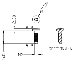
TORX HEAD SCREW
