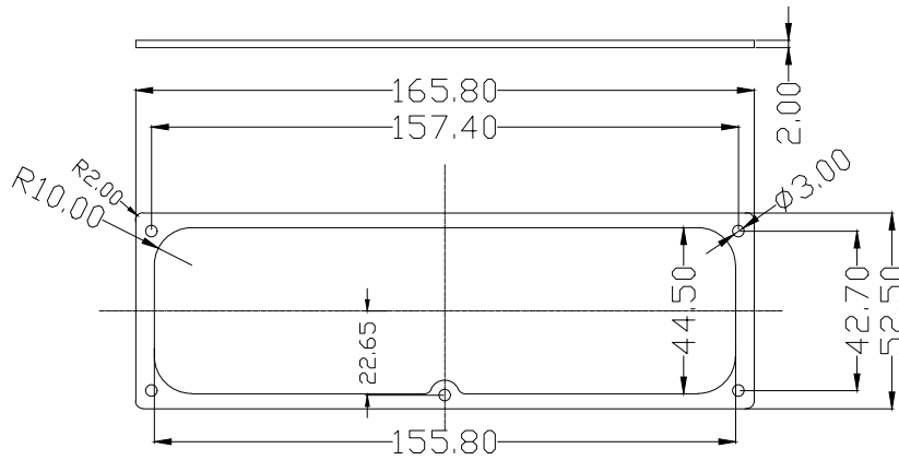
SK-4 SEALING KIT OPTIONAL ACCESSORY
