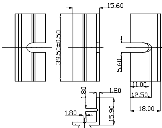
MF-40 OPTIONAL ACCESSORY
