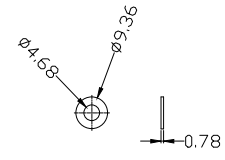
SEALING WASHERS
