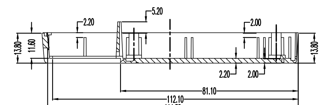
BOTTOM-SECTION
