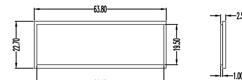
STANDARD END PLATE
