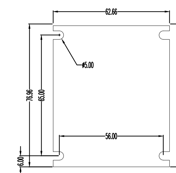
WITH BATTERY
