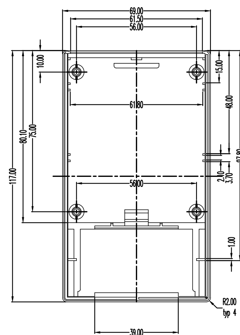
BOTTOM-INSIDE
