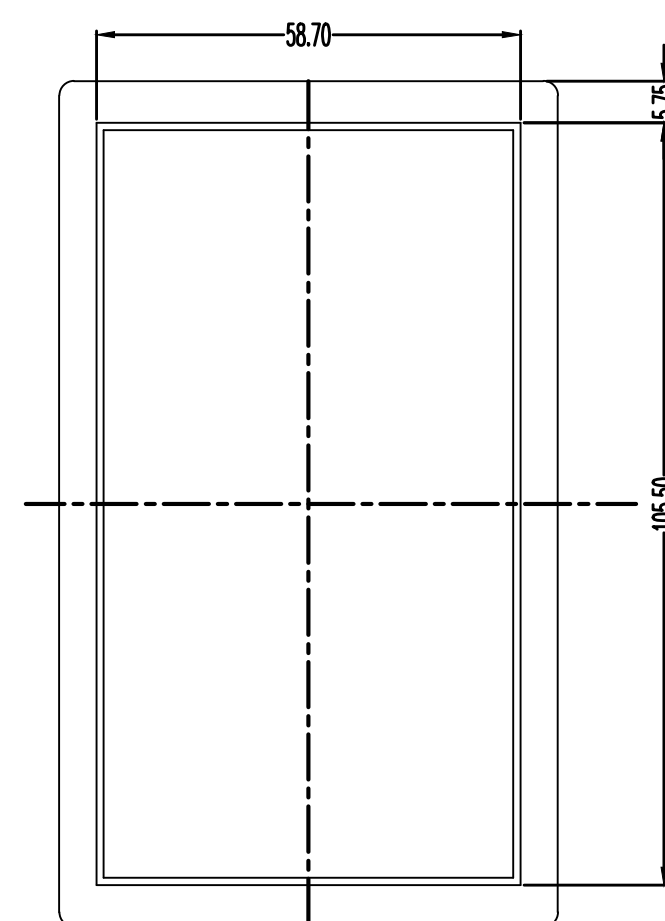
FLUSH TOP-OUTSIDE
