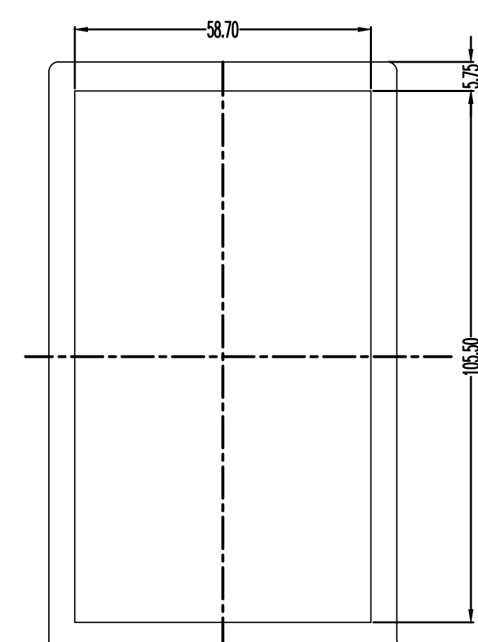
RECESSED TOP-OUTSIDE
