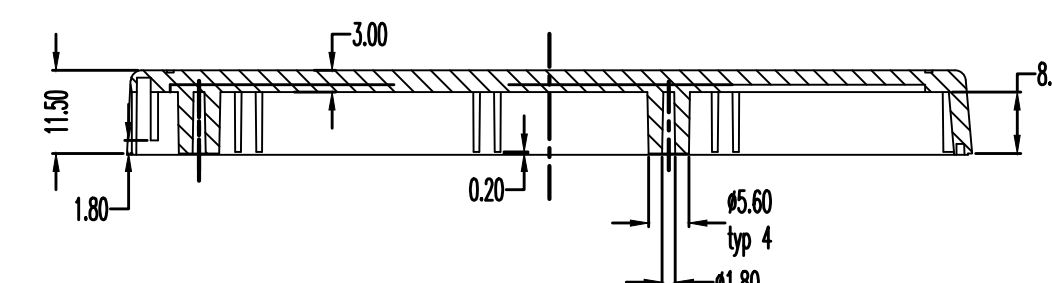
TOP-SECTION
