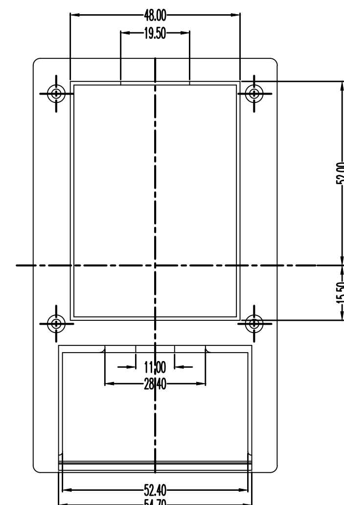
BOTTOM-OUTSIDE
