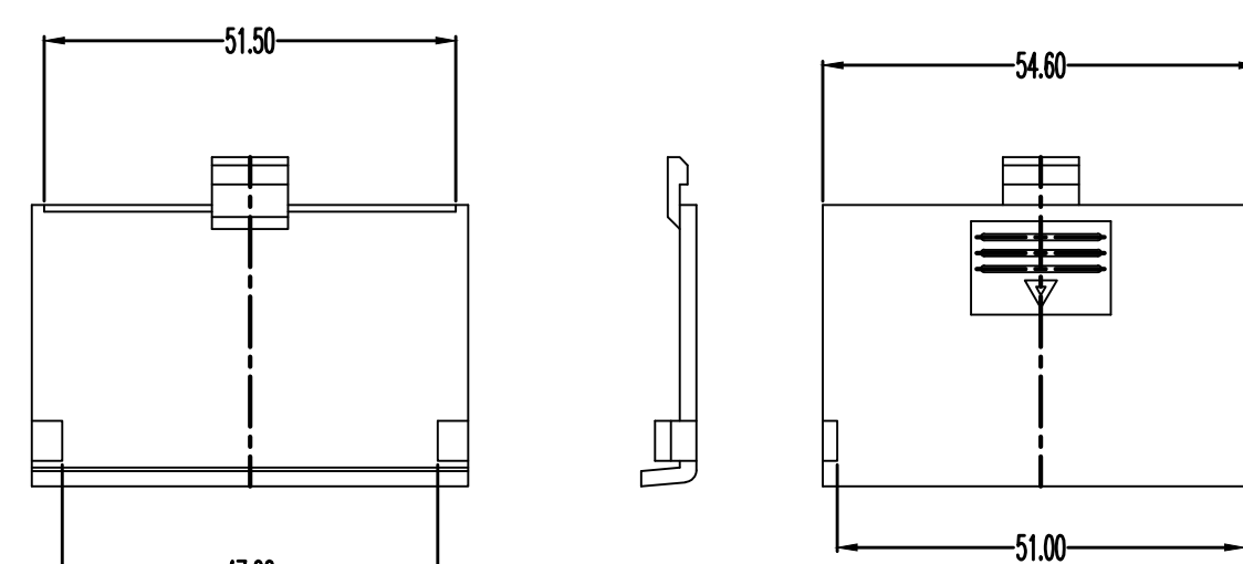
BATTERY DOOR
