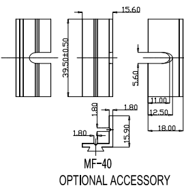
MF-40 OPTIONAL ACCESSORY
