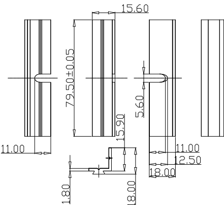
MF-80 OPTIONAL ACCESSORY
