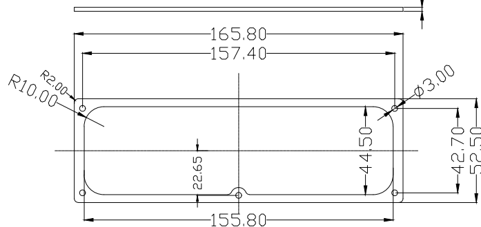
SK-4 SEALING KIT OPTIONAL ACCESSORY
