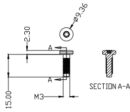
TORX HEAD SCREW
