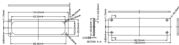
END PLATE
