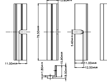
MF-80 OPTIONAL ACCESSORY
