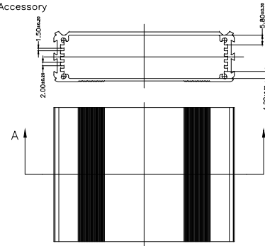
SK-2 SEALING KIT Optional Accessory
