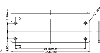
END PLATE
