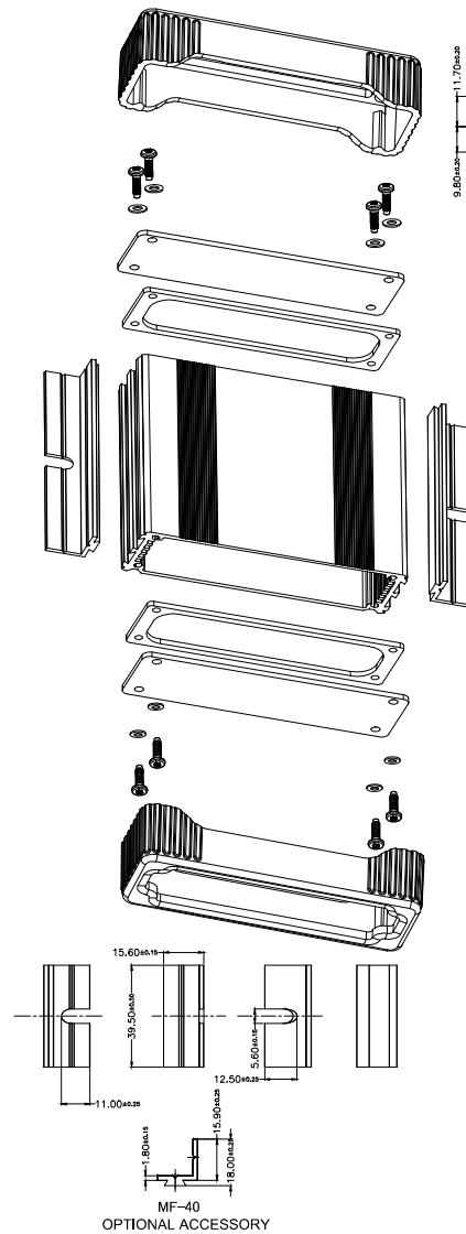
SK-2 SEALING KIT Optional Accessory
