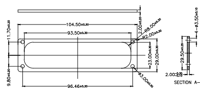
SK-2 SEALING KIT Optional Accessory
