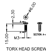
TORX HEAD SCREW
