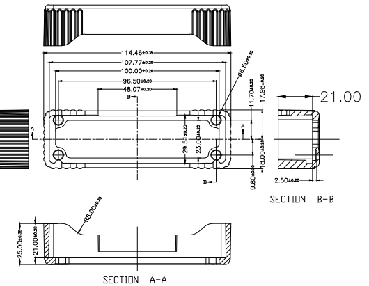
EC2 End Cap Optional Accessory
