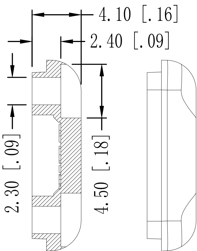
SECTION B-B
