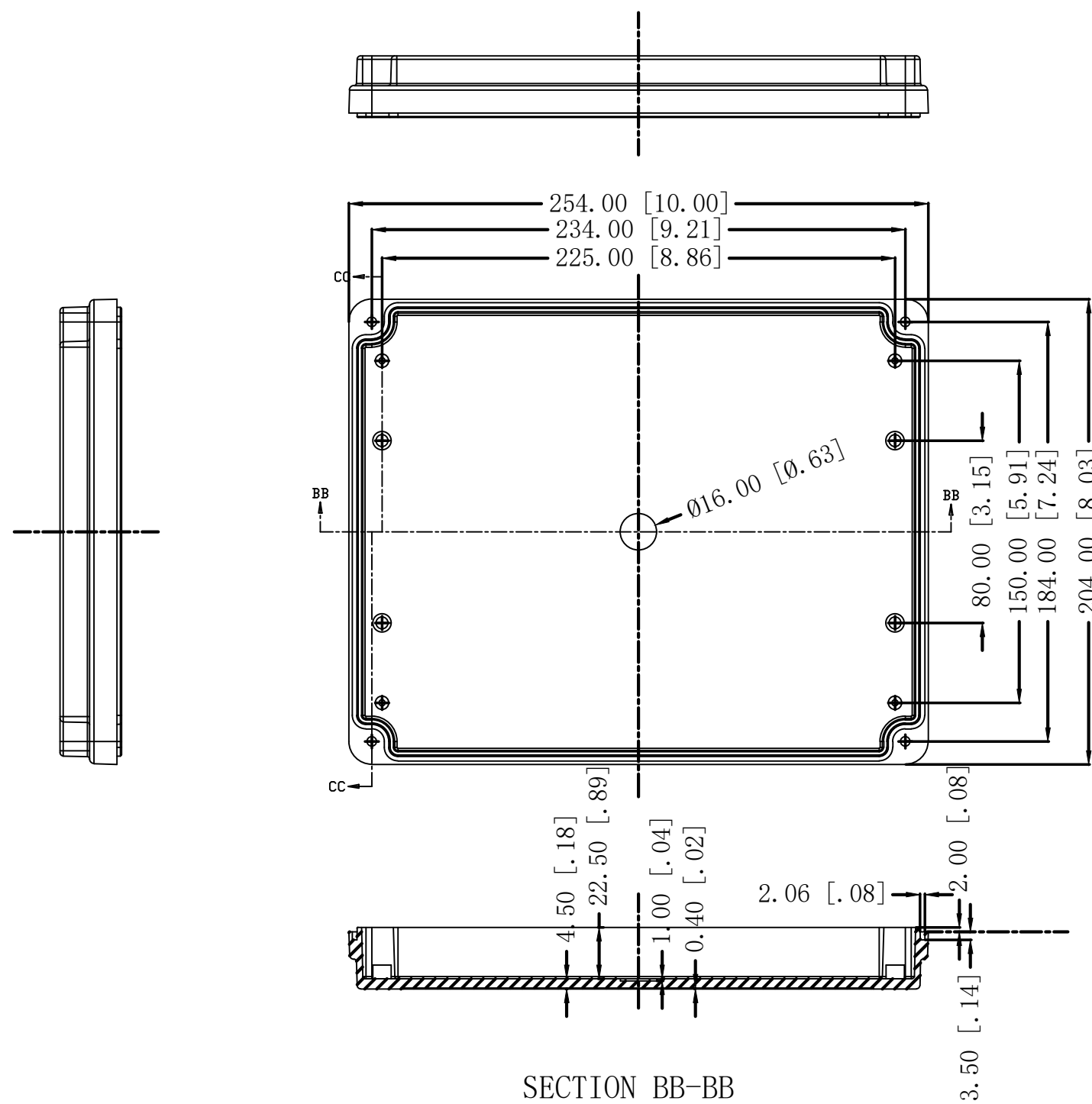
SECTION BB-BB
