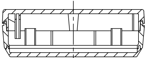
Section C-C
